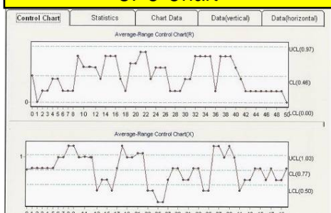
SPC Chart
