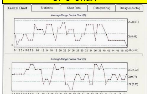
SPC Chart
